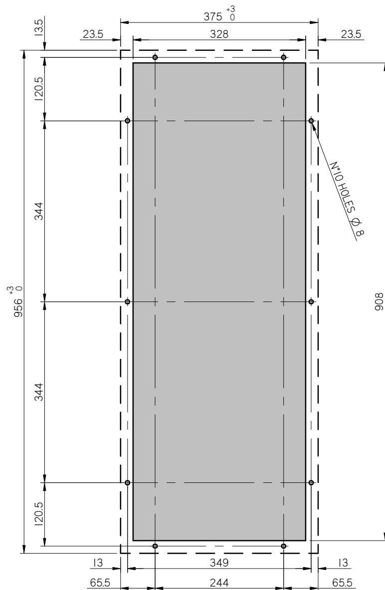
MONTAGGIO A INCASSO / SEMINCASSO FLUSH / SEMI-FLUSH MOUNTING
