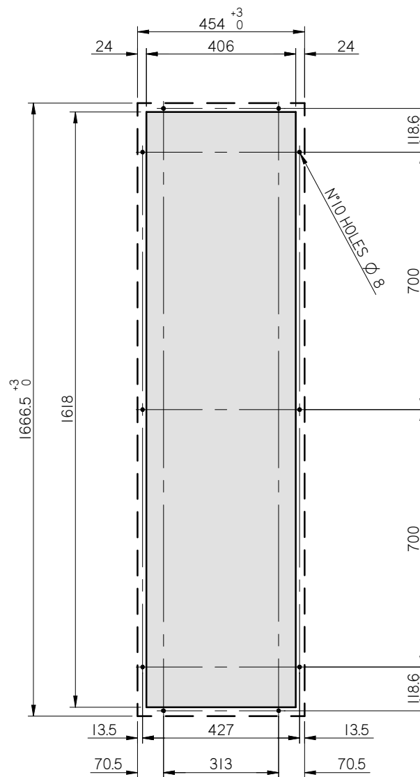
MONTAGGIO A INCASSO / SEMINCASSO FLUSH / SEMI-FLUSH MOUNTING
