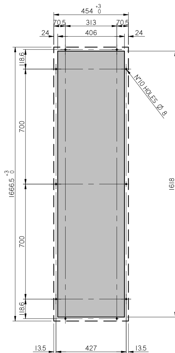
MONTAGGIO A INCASSO / SEMINCASSO FLUSH / SEMI-FLUSH MOUNTING
